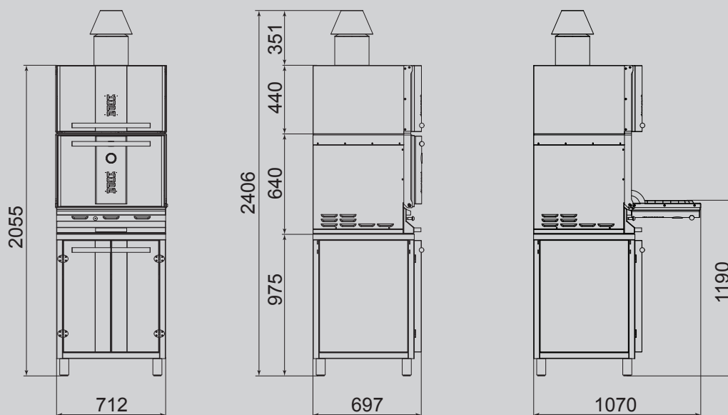
* Type 400SWC with wheels
